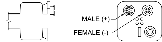
PDSN-13B SNAP TERMINAL
