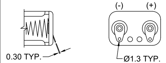
PDSN-36-2C SOLDER LUGS
