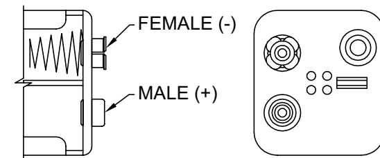
PDSN-38-2B SNAP TERMINAL
