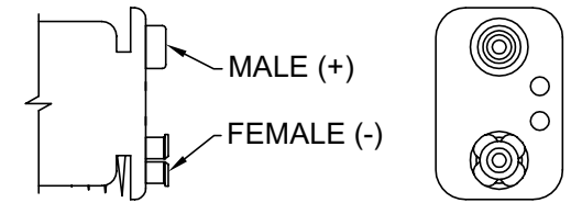
PDSN-36-2B SNAP TERMINAL
