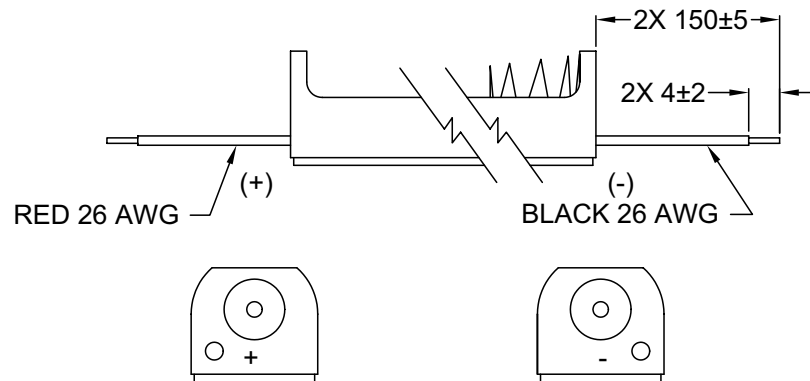
PDSN-12A WIRE LEADS
