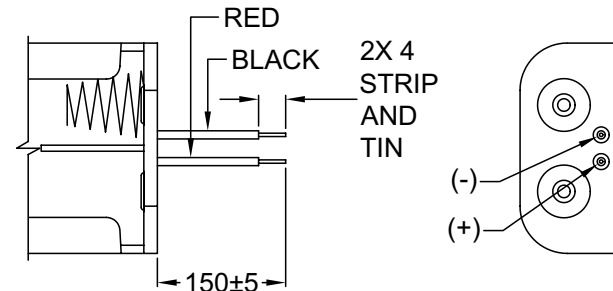
PDSN-11A WIRE LEADS
