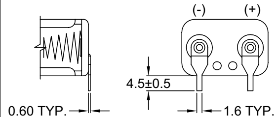
PDSN-36-2D PCB PINS
