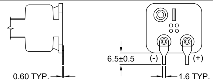
PDSN-13D PCB PINS
