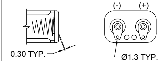
PDSN-22C SOLDER LUGS
