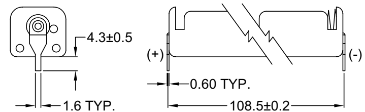
PDSN-19D PCB PINS
