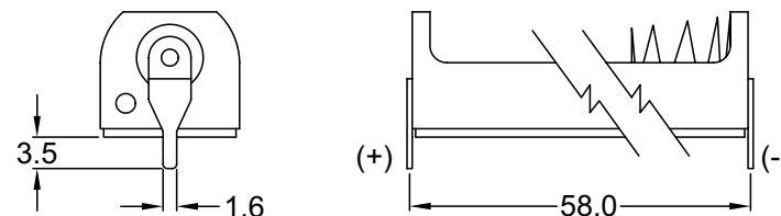
PDSN-12D P.C. PINS
