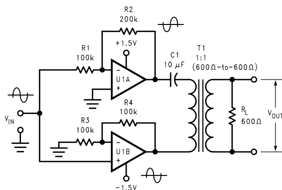
Figure 43. Differential Driver
