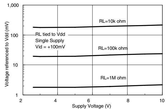
Figure 8. High level output voltage vs. supply voltage
