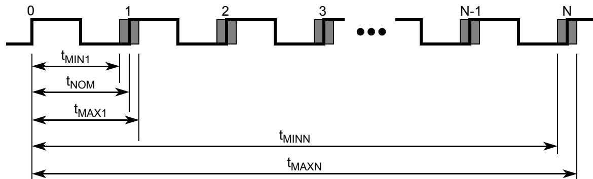
Figure 10. Jitter Definitions
