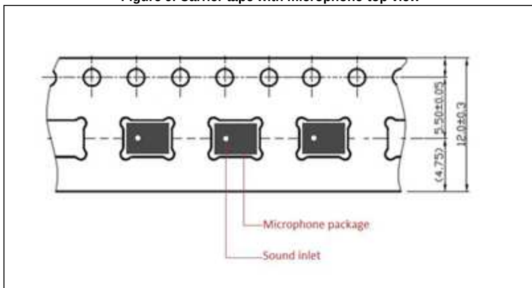
Figure 9. Carrier tape with microphone-top view
