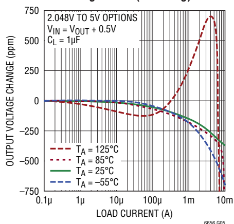
Load Regulation (Sourcing)
