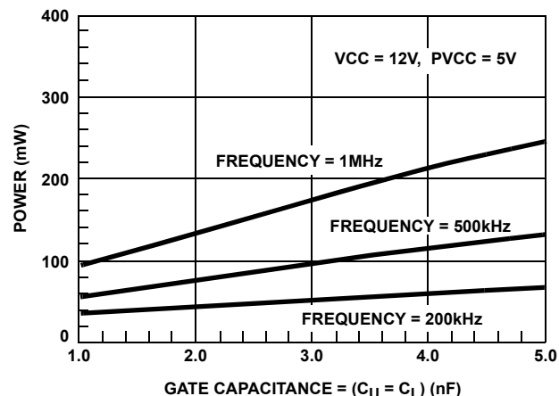
FIGURE 6. VARIABLE LOADING PROFILE (HIP6603B)
