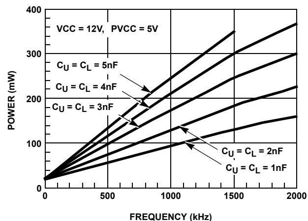
FIGURE 4. POWER DISSIPATION vs FREQUENCY (HIP6603B)
