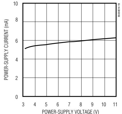
POWER-SUPPLY CURRENT (PER AMPLIFIER) vs. POWER-SUPPLY VOLTAGE
