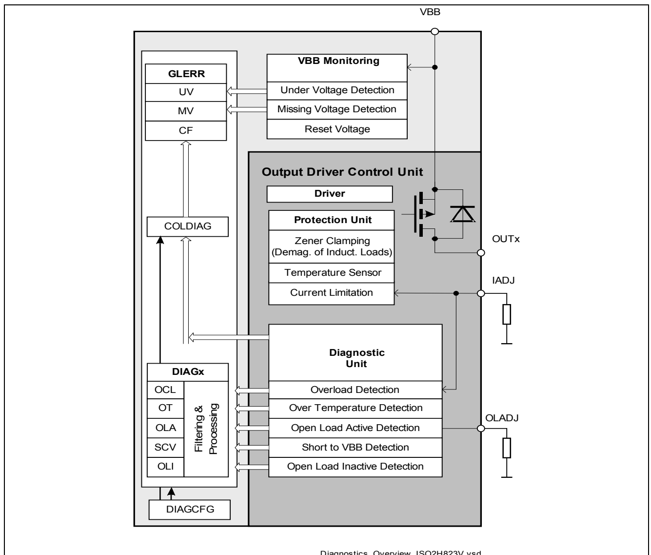
Figure 21 Diagnostics Overview
