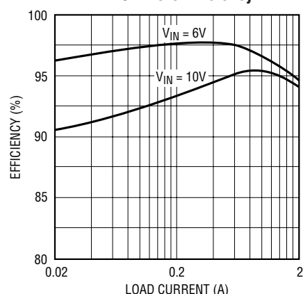
LTC1148-5 Efficiency
