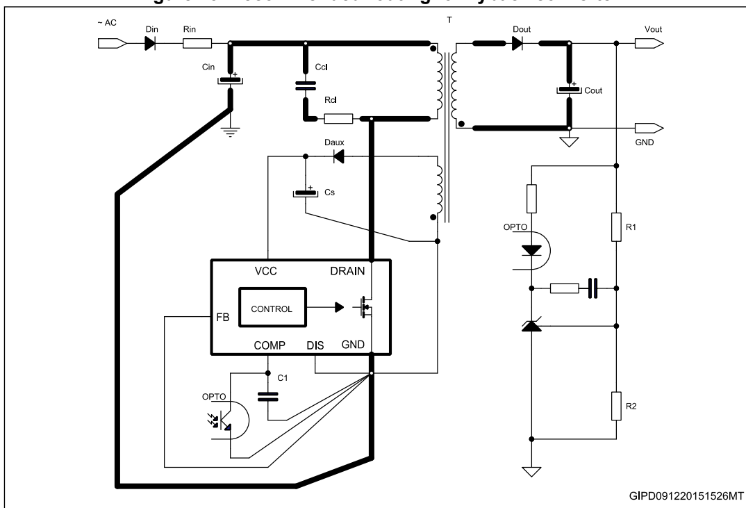
Figure 45. Recommended routing for flyback converter
