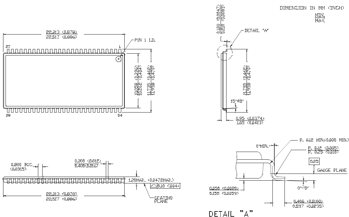
54-lead Thin Small Outline Package, Type II Z54-II
