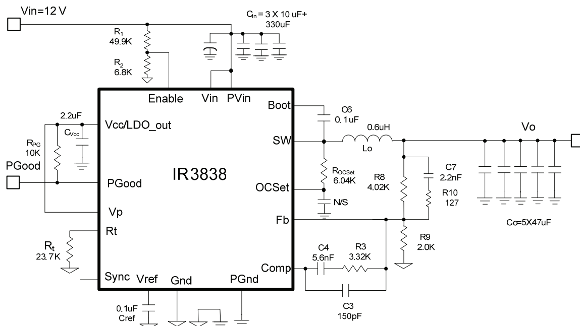
Fig. 21. Application circuit diagram for a 12V to 1.8 V, 10 A Point Of Load Converter
