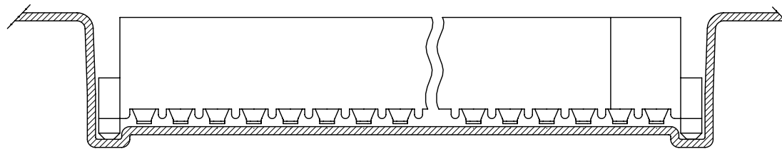
SECTION B-B
