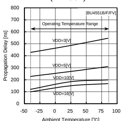
Fig.45 propagation delay time tPHZ (CONT—OUT)
