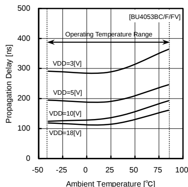
Fig.33 propagation delay time tPZH (CONT—OUT)
