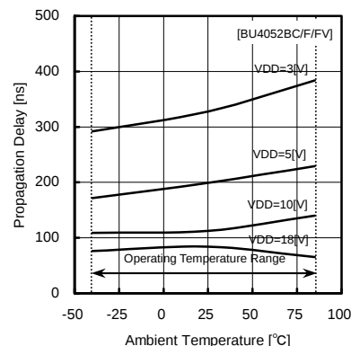
Fig.24 propagation delay time tPLZ (CONT—OUT)
