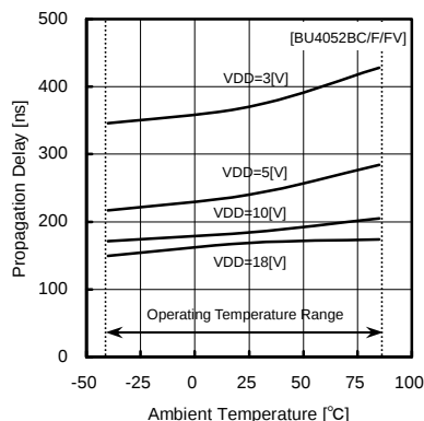
Fig.22 propagation delay time tPZH (CONT—OUT)
