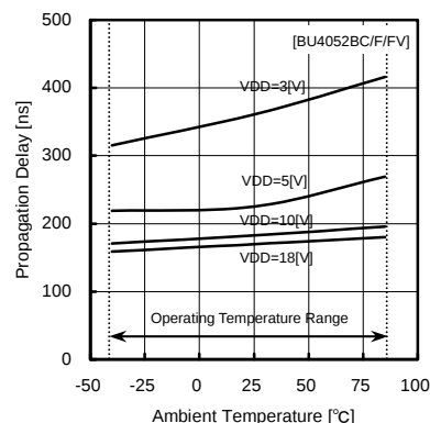
Fig.27 propagation delay time tPHZ (INH—OUT)
