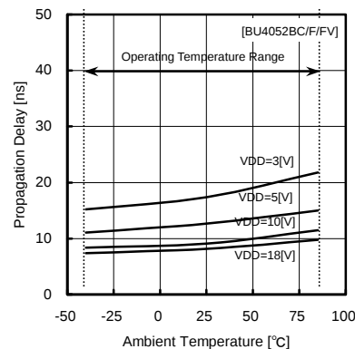
Fig.21 propagation delay time tPHL (IN—OUT)
