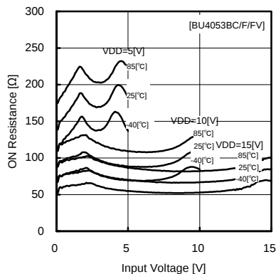
Fig.30 ON resistance—input voltage
