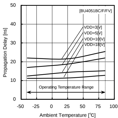
Fig.9 propagation delay time tPLH (IN – OUT)
