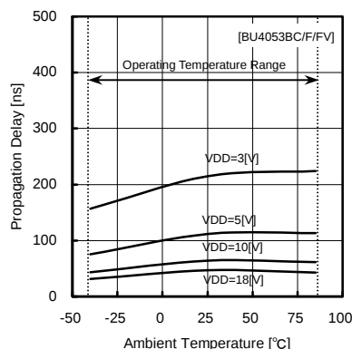
Fig.36 propagation delay time tPZL (CONT—OUT)
