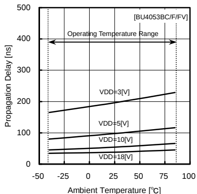
Fig.40 propagation delay time tPLZ (INH—OUT)
