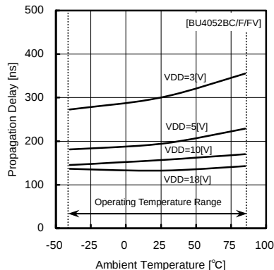
Fig.28 propagation delay time tPZL (INH—OUT)
