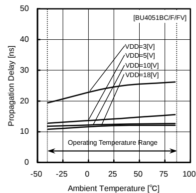
Fig.10 propagation delay time tPHL (IN – OUT)
