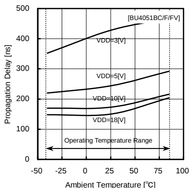
Fig.12 propagation delay time tPHZ (CONT – OUT)
