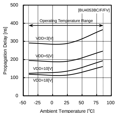
Fig.34 propagation delay time tPHZ (CONT—OUT)
