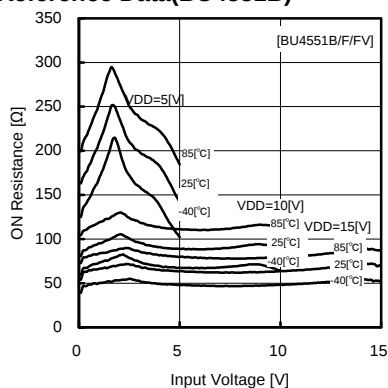
Fig.41 ON resistance—input voltage
