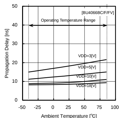
Fig.3 falling propagation delay (IN – OUT)
