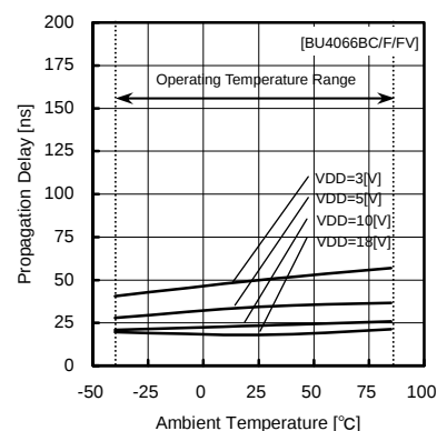
Fig.6 rising propagation delay (CONT – OUT ,tPLZ)
