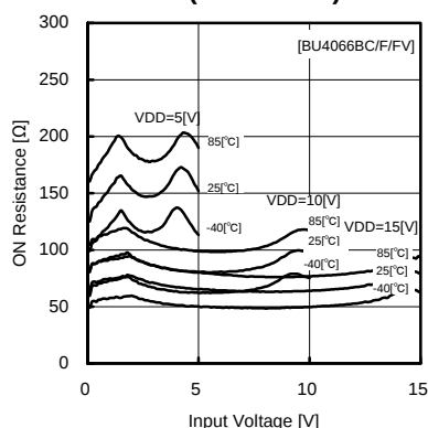
Fig.1 On resistance – input voltage
