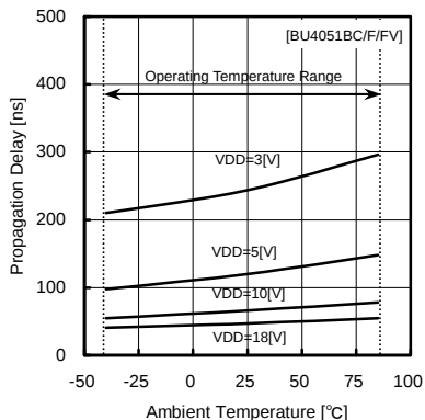
Fig.18 propagation delay time tPLZ (INH – OUT)
