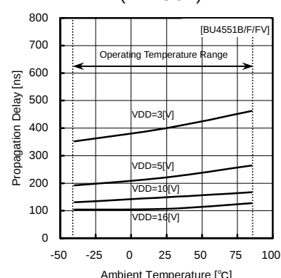
Fig.46 propagation delay time tPLZ (CONT—OUT)
