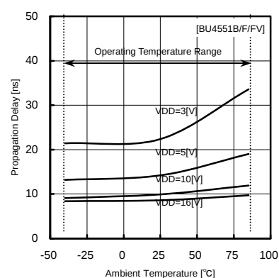
Fig.43 propagation delay time tPHL (IN—OUT)
