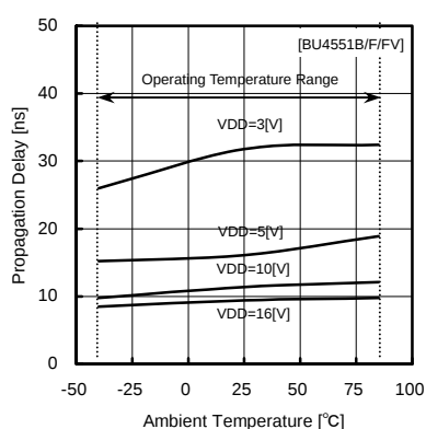
Fig.42 propagation delay time tPLH (IN—OUT)
