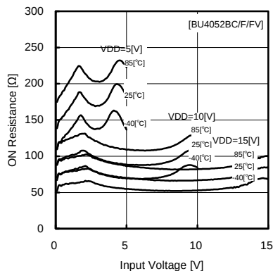
Fig.19 ON resistance—input voltage
