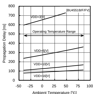
Fig.47 propagation delay time tPZL (CONT—OUT)
