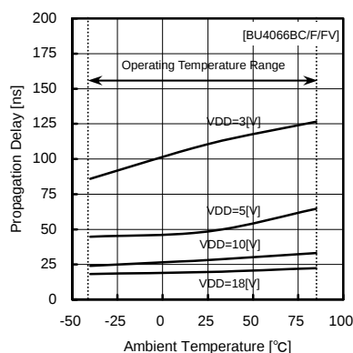
Fig.4 rising propagation delay (CONT – OUT ,tPZH)
