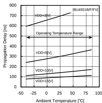
Fig.44 propagation delay time tPZH (CONT—OUT)
