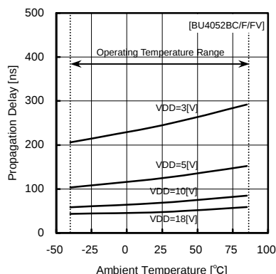
Fig.25 propagation delay time tPZL (CONT—OUT)
