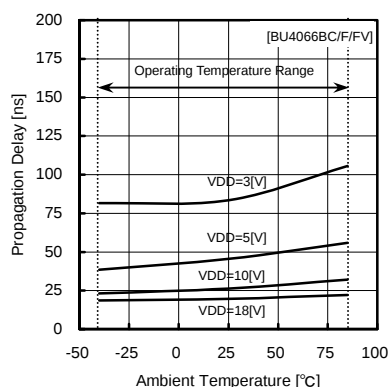
Fig.7 falling propagation delay (CONT – OUT ,tPZL)
