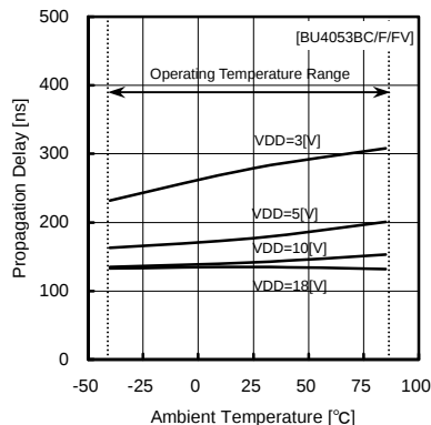
Fig.39 propagation delay time tPZL (INH—OUT)
