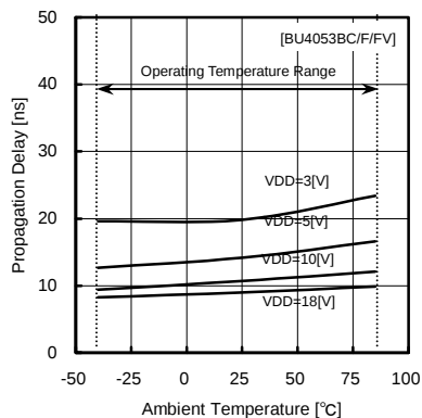
Fig.31 propagation delay time tPLH (IN—OUT)
