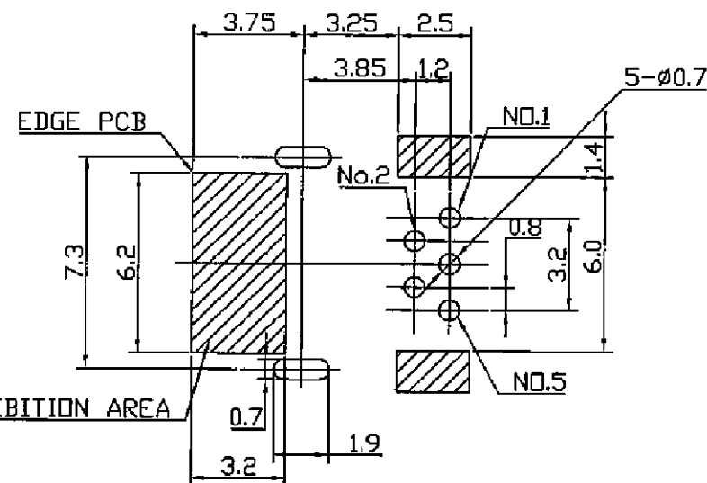
RECOMMENDED PCB PATTERN LAYOUT (PCB THICKNESS: 0.8 \pm 0.1 )
