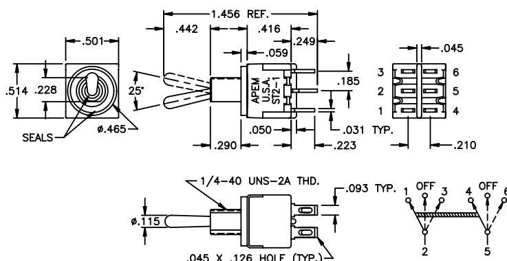
DOUBLE POLE
