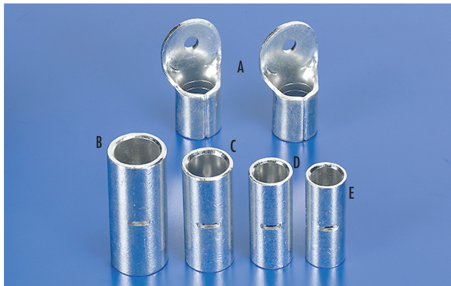
Large Brazed-Seam Terminals: A = 400 MCM Wire Gauge Large Brazed-Seam Splices: B = 500 to 600 MCM Wire Gauge, C = 350 to 450 MCM Wire Gauge D = 300 to 350 MCM Wire Gauge, E = 250 to 300 MCM Wire Gauge
