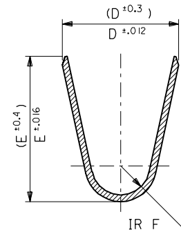
SECT. H-H
