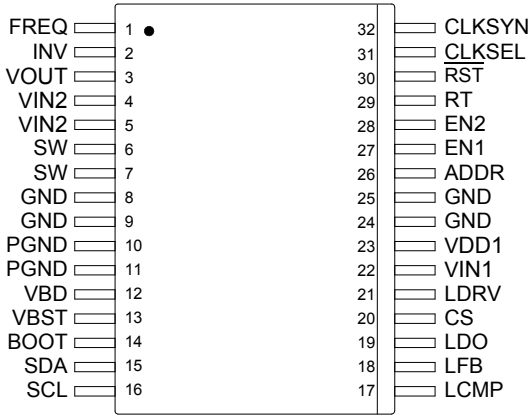
Figure 3. Pin Connections
