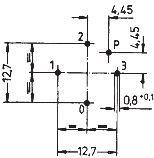
PCB hole pattern, sight on component side
