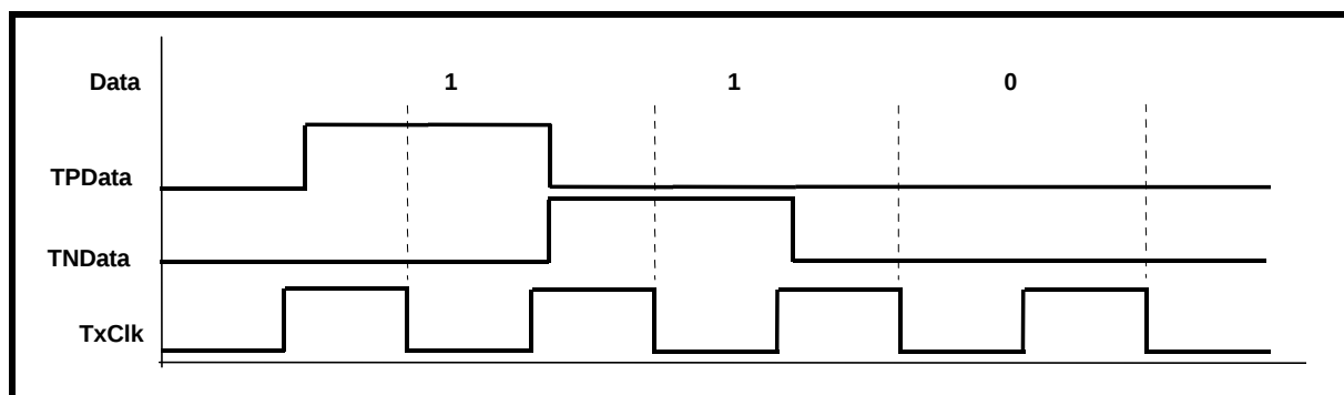
FIGURE 15. THE XRT73LC03A SAMPLES THE DATA ON THE TPDData AND TNDData INPUT PINS
