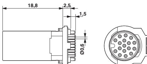
M12 plug, straight, shielded,
