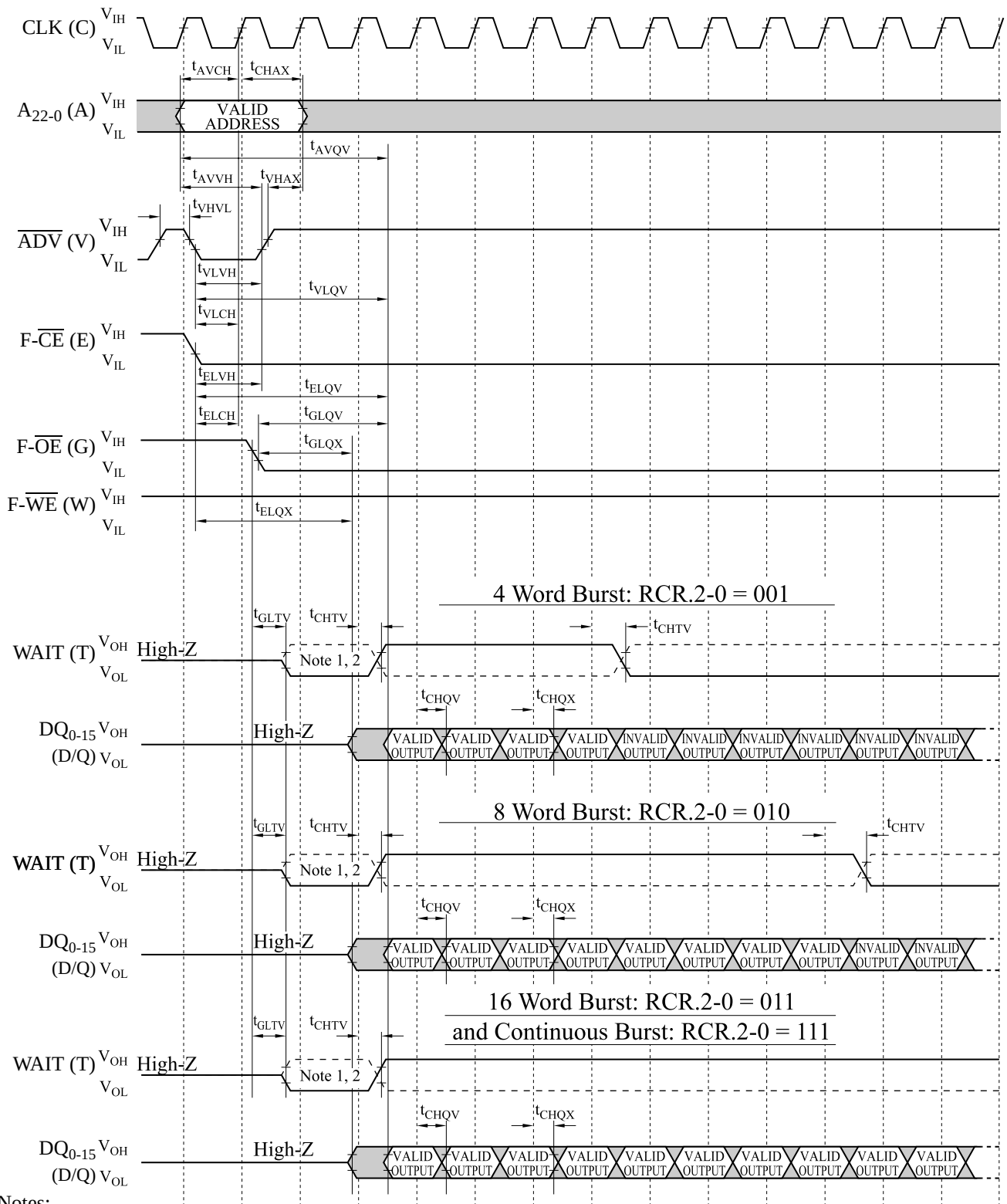
AC Waveform for Synchronous Burst Mode Read Operations from Main Blocks or Parameter Blocks (Frequency Configuration: RCR.13-11=010)
