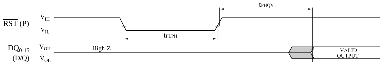
(A) Reset during Read Array Mode
