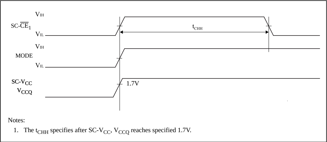
Power-Up Initialization Timing
