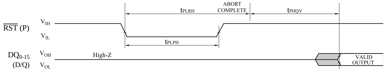
(B) Reset during Erase or Program Mode
