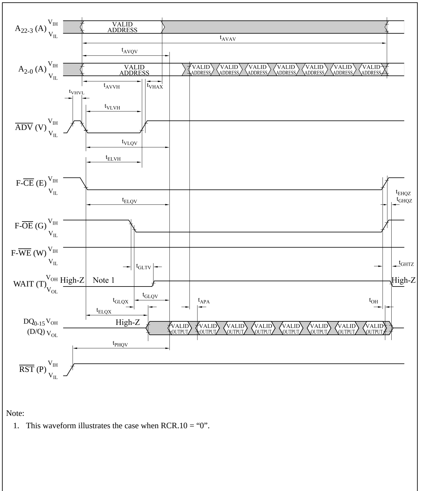
AC Waveform for Asynchronous 8-Word Page Mode Read Operations from Main Blocks or Parameter Blocks
