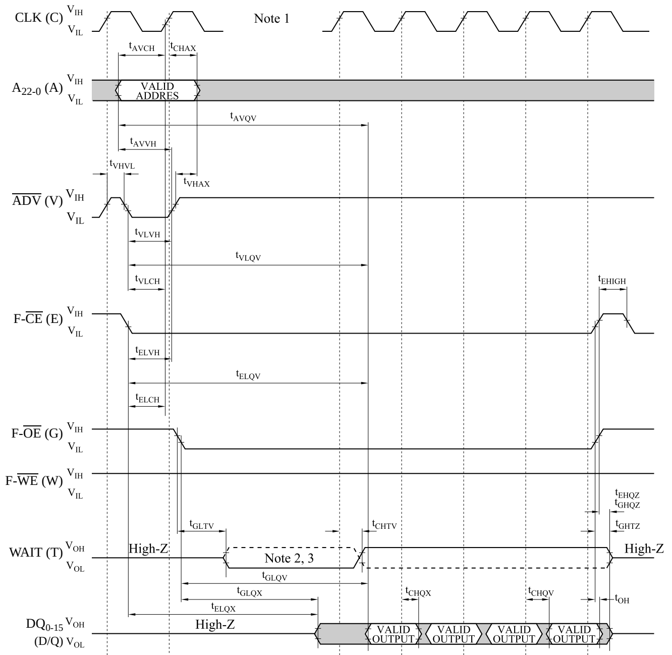
AC Waveform for Synchronous Burst Mode Read Operations from Main Blocks or Parameter Blocks (4 Word Burst: RCR.2-0=001)
