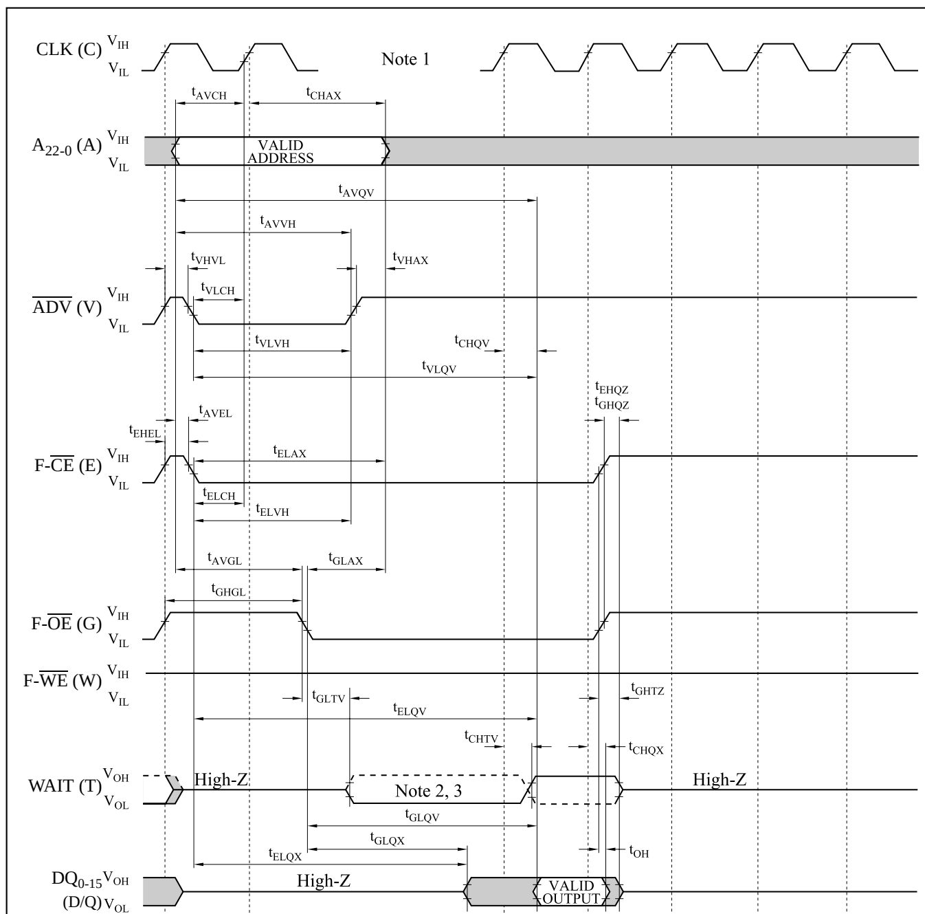
AC Waveform for Single Synchronous Read Operations from Status Register, Identifier Codes, OTP Block or Query Code
