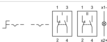
Wiring diagram 26
