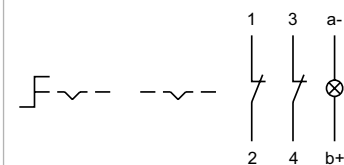
Wiring diagram 18
