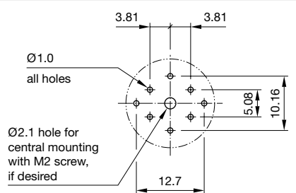
Component layout 1
