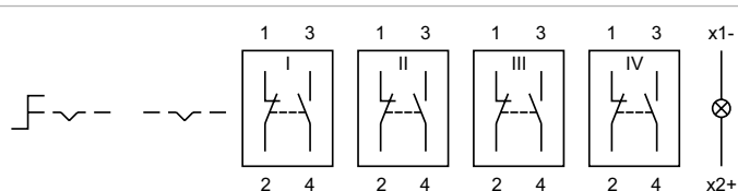
Wiring diagram 28
