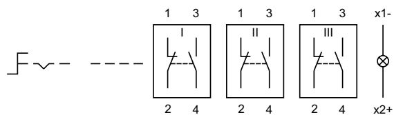
Wiring diagram 13
