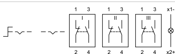
Wiring diagram 27
