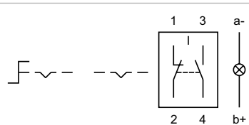
Wiring diagram 23
