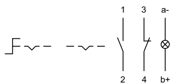
Wiring diagram 16
