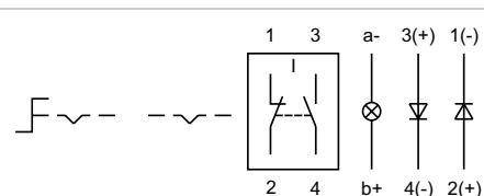
Wiring diagram 21
