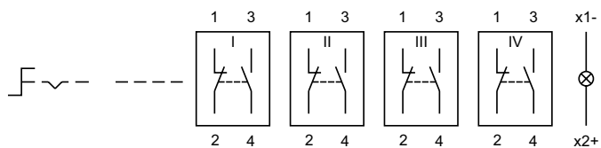
Wiring diagram 14
