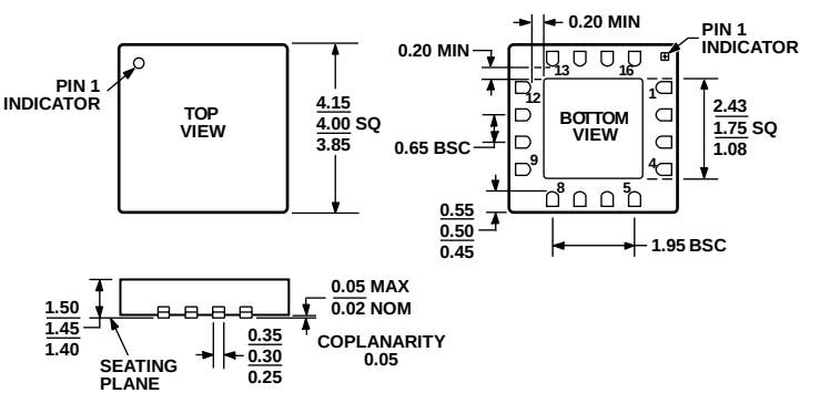
Figure 21. 16-Lead Lead Frame Chip Scale Package [MQ_LFCSP_LQ] 4 mm x 4 mm Body, Thick Quad (CP-16-5a*) Dimensions shown in millimeters (Drawing Not to Scale)
