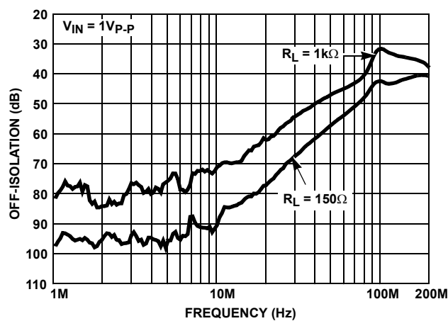
FIGURE 15. ALL HOSTILE OFF-ISOLATION
