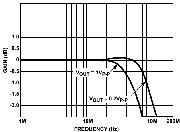
FIGURE 13. GAIN FLATNESS
