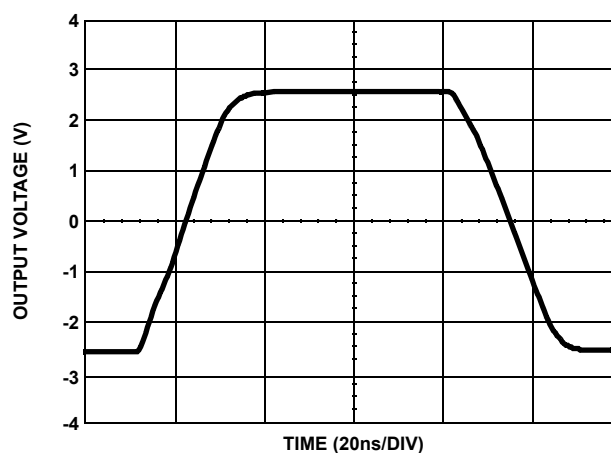
FIGURE 11. LARGE SIGNAL PULSE RESPONSE
