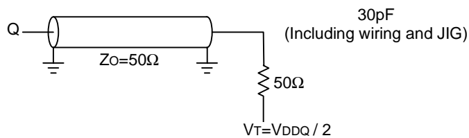
Fig.1 Output load
