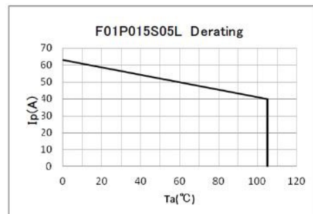
Figure 4: I_p vs T_a for F01P015S05L
