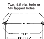
Mounting Holes
