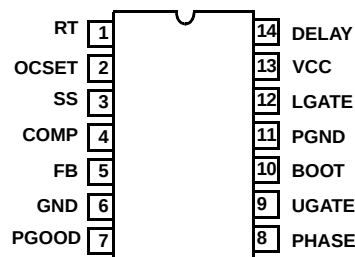
ISL6525 (SOIC) TOP VIEW
