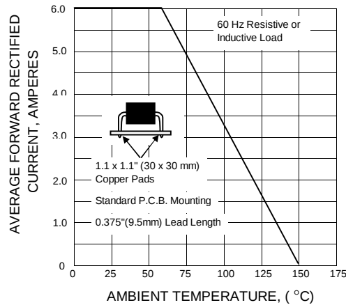
FIG.1 - MAXIMUM FORWARD CURRENT DERATING CURRENT
