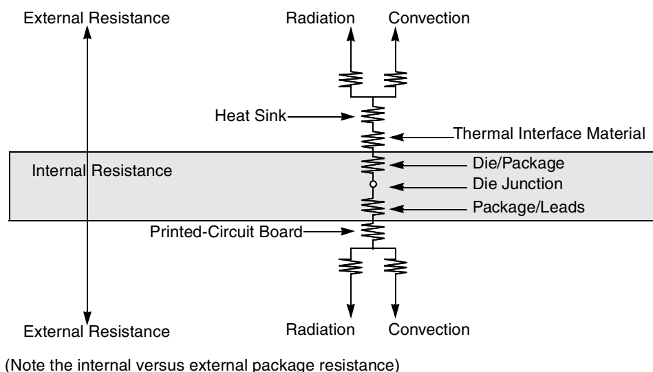
Figure 30. PBGA Package with Heat Sink Mounted to a Printed-Circuit Board
