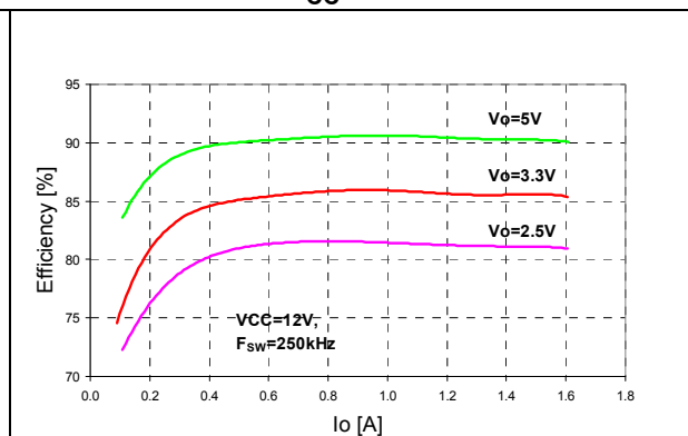
Figure 25. Efficiency vs. output current - V_{CC} = 12\text{ V}
