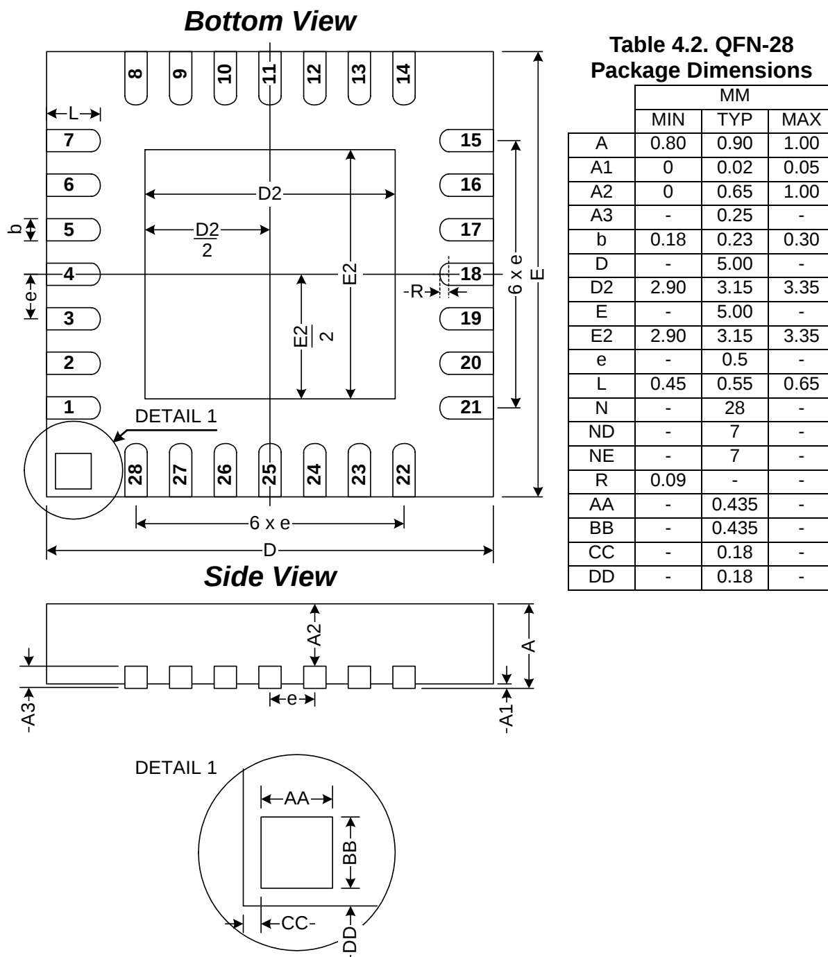
Figure 4.3. QFN-28 Package Drawing
