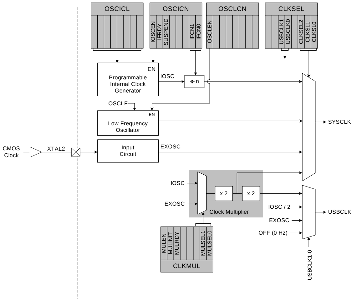
Figure 10.1. Oscillator Diagram
