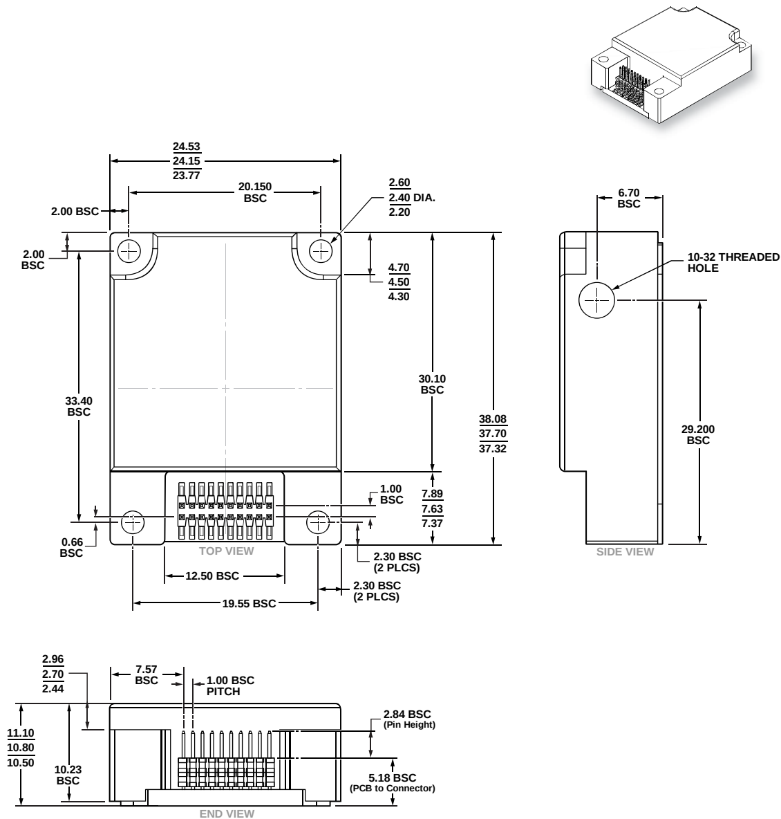
Figure 26. 20-Lead Module with Connector Interface (ML-20-2) Dimensions shown in millimeters
