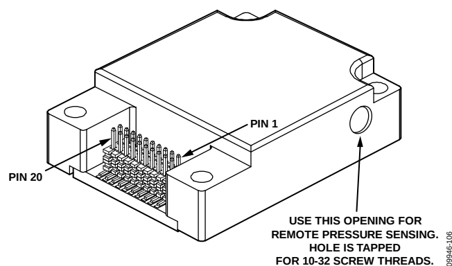
Figure 6. Pin Locations
