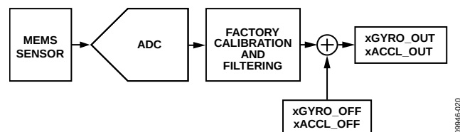
Figure 21. User Calibration, Gyroscopes, and Accelerometers
