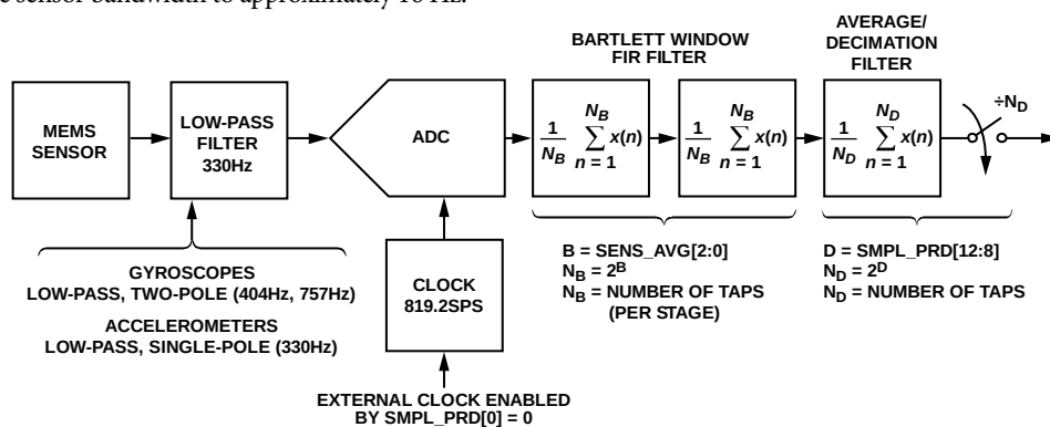
Figure 20. Sampling and Frequency Response Block Diagram
