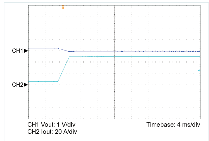
Figure 8 — 10% to 100% load transient response, V_{IN} = 270\text{ V} , nominal trim, C_{OUT\_EXT} = 1000\text{ }\mu\text{F}
