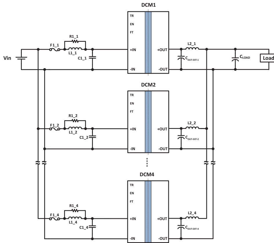
Typical Application 1: DCM4623xD2K06B5yzz in an array of four units
