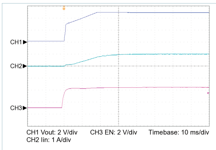
Figure 17 — Startup from EN, V_{IN} = 270\text{ V} , C_{OUT\_EXT} = 10000\text{ }\mu\text{F} , R_{LOAD} = 0.100\text{ }\Omega
