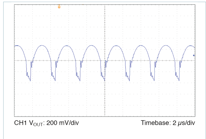
Figure 19 — Output voltage ripple, V_{IN} = 270\text{ V} , V_{OUT} = 5.0\text{ V} , C_{OUT\_EXT} = 1000\text{ }\mu\text{F} , R_{LOAD} = 0.100\text{ }\Omega
