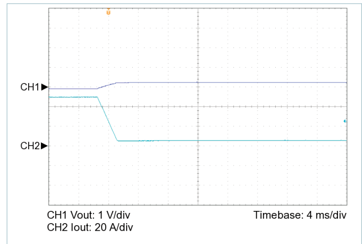
Figure 7 — 100% to 10% load transient response, V_{IN} = 270\text{ V} , nominal trim, C_{OUT\_EXT} = 1000\text{ }\mu\text{F}
