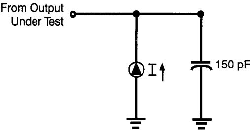
Figure 5. Test Load Diagram
