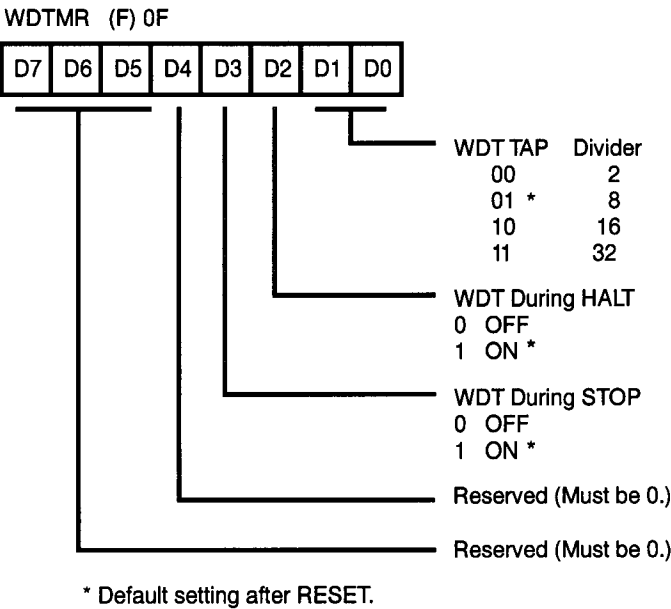
Figure 17. WDT Mode Register
