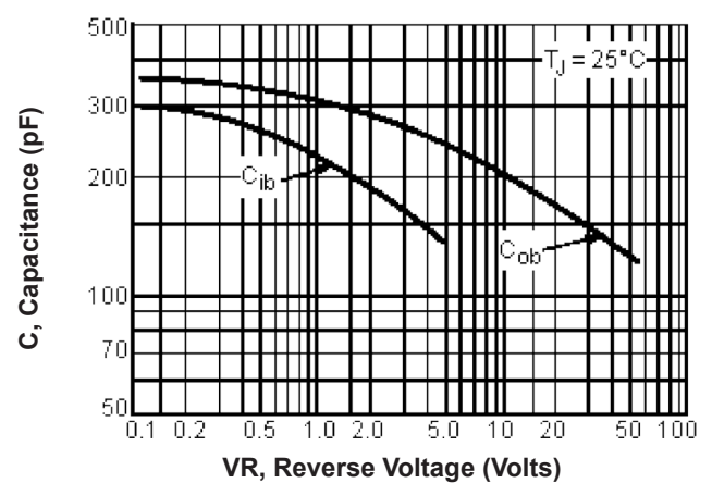
Capacitance
