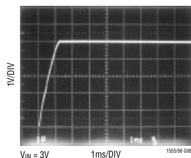
V_{CC} Output Voltage Turn-On Time, SS Disabled
