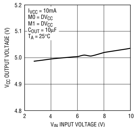
V_{CC} Output Voltage vs Input Voltage (5V Mode)
