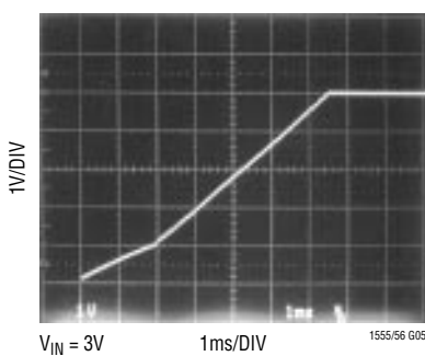
V_{CC} Output Voltage Turn-On Time, SS Enabled
