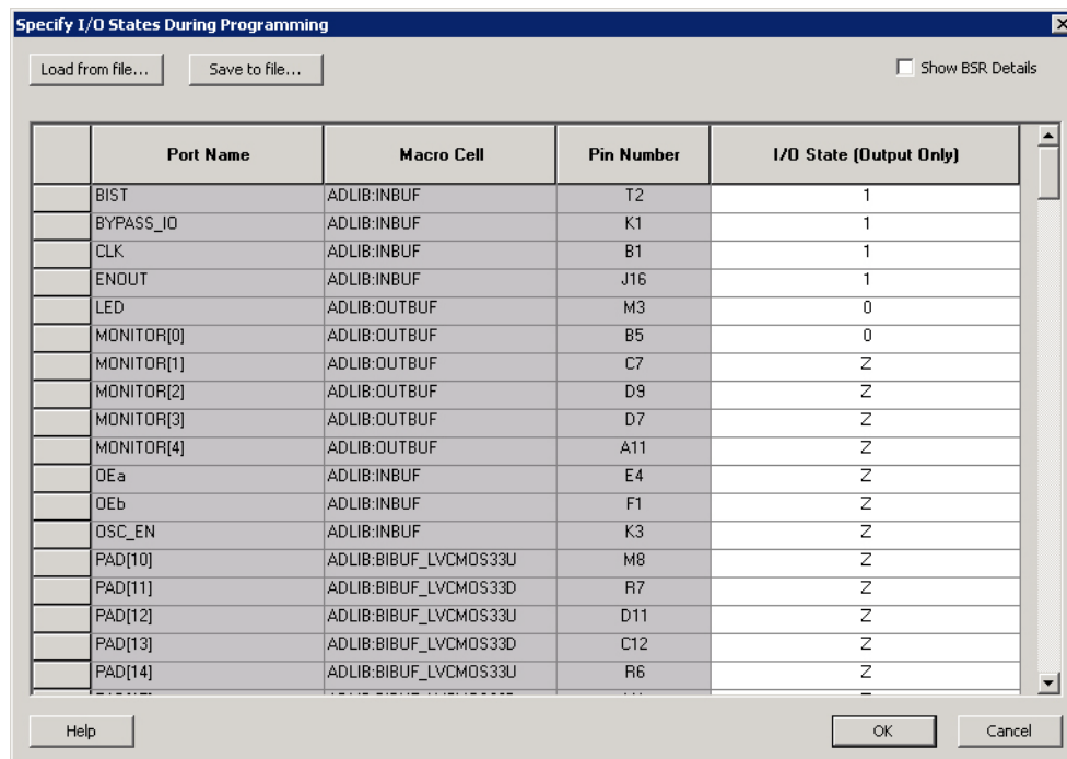
Figure 1-3 • I/O States During Programming Window
