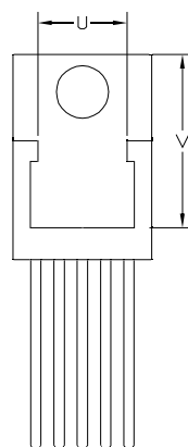
Btm View
