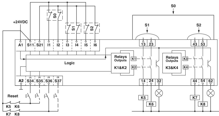
Circuit diagram
