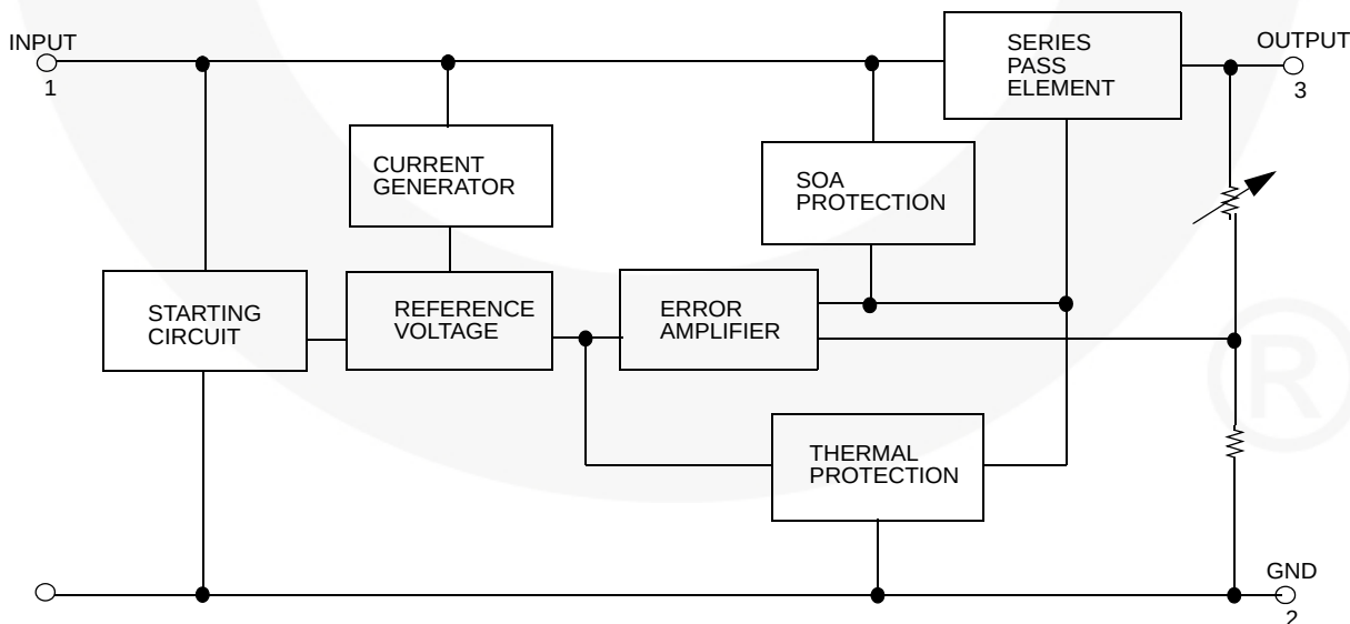
Figure 1. Block Diagram
