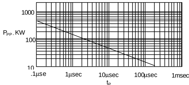
Peak Pulse Power ( P_{PP} ) – versus – Pulse Time ( t_P )
