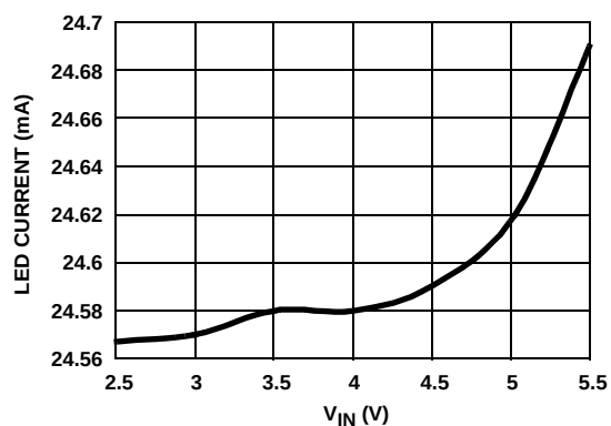
FIGURE 4. LINE REGULATION
