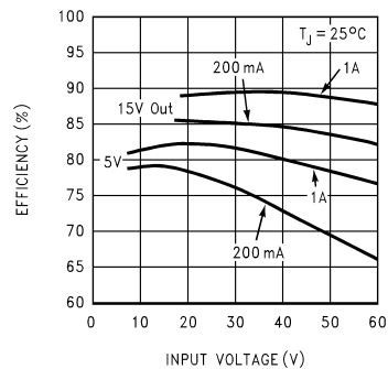
Efficiency
