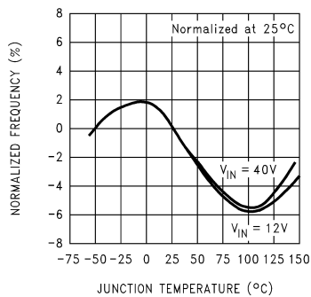
Oscillator Frequency
