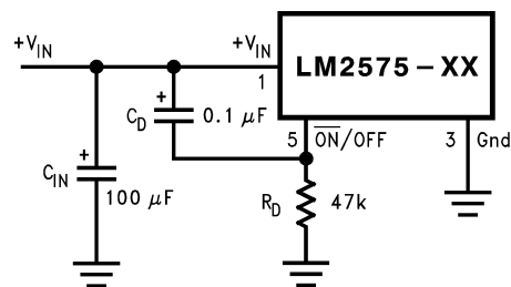
FIGURE 13. Undervoltage Lockout for Buck-Boost Circuit
