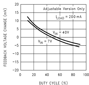
Feedback Voltage vs Duty Cycle
