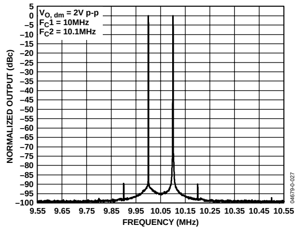
Figure 33. Intermodulation Distortion
