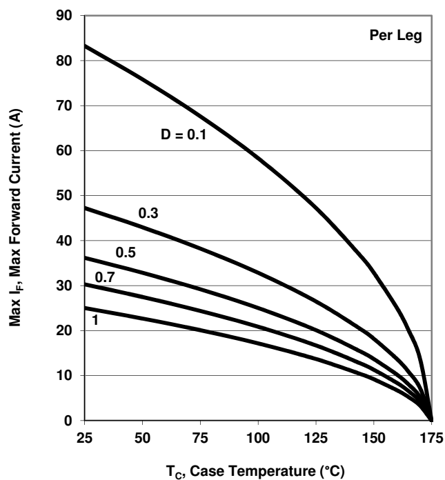
Figure 3. Max Forward Current I_F = f(T_C) ; T_j = 175^{\circ}\text{C} ; R_{th,JC(max)}
