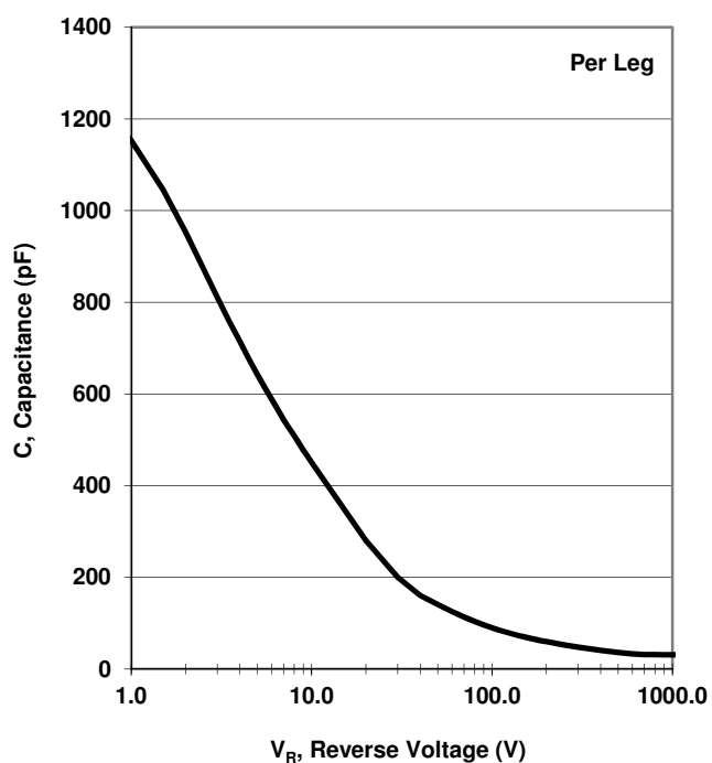
Figure 4. Typ. Capacitance vs. Reverse Voltage C = f(V_R) ; T_C = 25^{\circ}\text{C} ; f = 1\text{ MHz}
