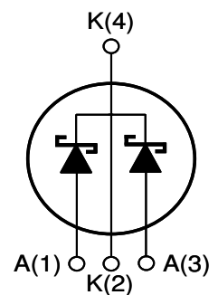
Internal Schematic
