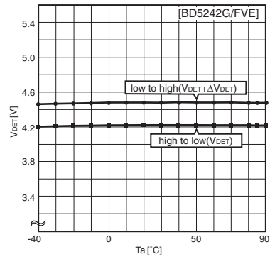
Detection voltage
